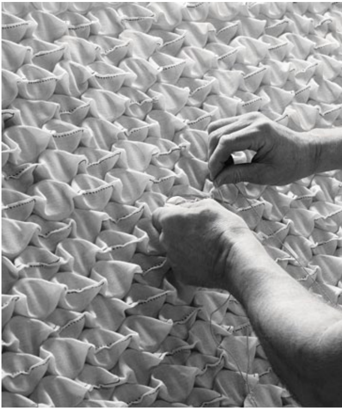
Hand-nesting the pocket springs.
